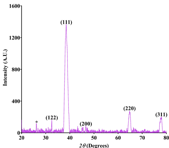
Fig. 3 X-ray diffraction pattern of the SS-AgNPs.
