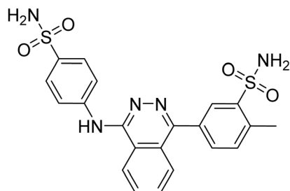
2-Methyl-5-(4-((4-sulfamoylphenyl)amino)phthalazin-1-yl)benzenesulfonamide
