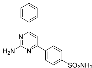
4-(2-amino-6-phenylpyrimidin-4-yl)benzenesulfonamide
