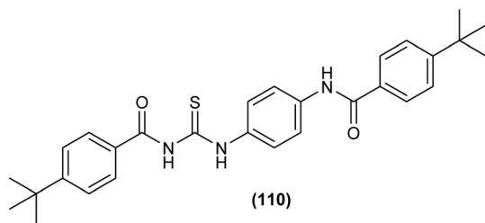
Fig. 44 Structure of 4-( tert -butyl)- N -((4-(4-( tert -butyl)benzamido)phenyl)carbamoithioyl) benzamide.
