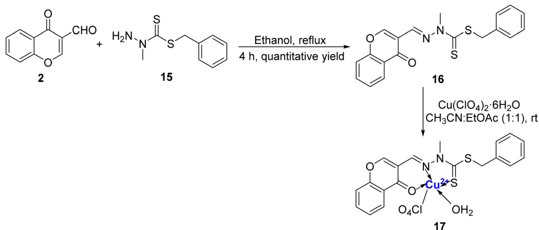
Scheme 5 Synthesis of ligand 16 and its complex 17 with Cu 2+ ion.
