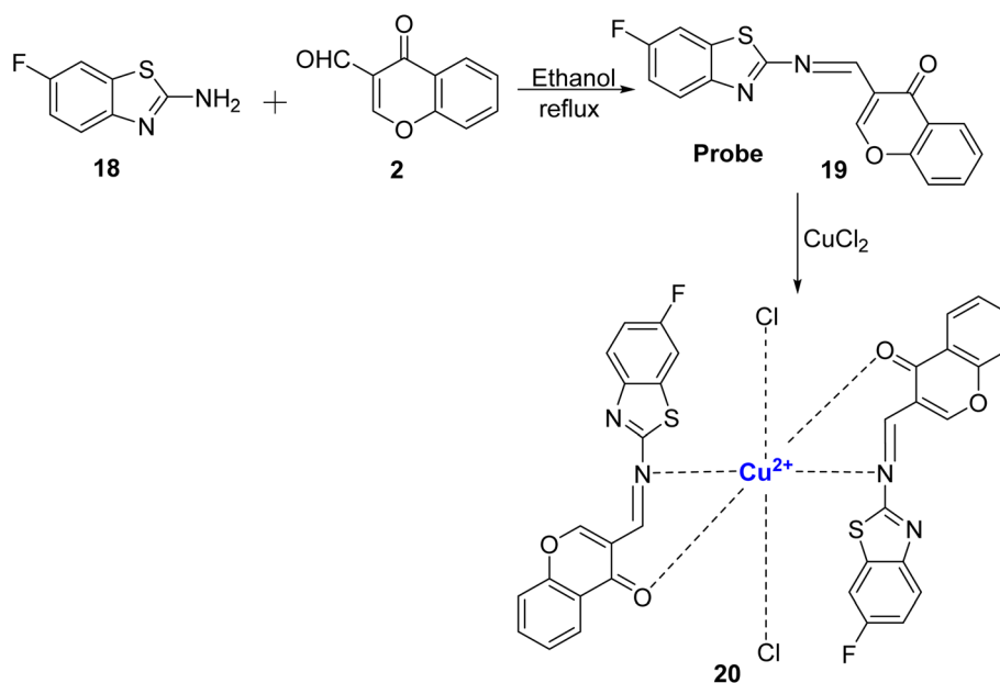
Scheme 6 Synthesis of chemosensor probe 19 and its complex with Cu 2+ ion 20 .
