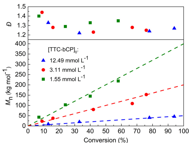
Fig. 2 Evolution of M_n and D during PI-RAFT polymerisation of MMA for different targeted molar masses. Dashed lines represent the theoretical molar masses.
