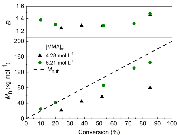
Fig. 1 Evolution of M_n and D during PI-RAFT polymerisation at ambient temperature with different concentrations of MMA in acetonitrile.
