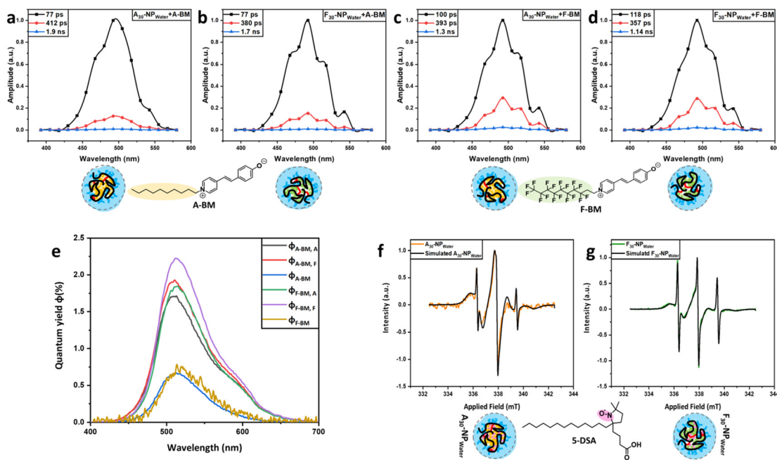
Fig. 3 DAS of A-BM in (a) A 30 -NP water and (b) F 30 -NP water ; DAS of F-BM in (c) A 30 -NP water and (d) F 30 -NP water . (e) Emission spectra of A-BM and F-BM. CW-EPR spectra and simulations of 5-DSA in the core of (f) A 30 -NP water and (g) F 30 -NP water .
