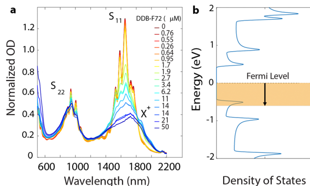
Fig. 1 (a) Absorption spectra of DDB-F72 doped s-SWCNT. Undoped sample (dark red, 0 μM DDB-F72) transitions to the highly doped sample (dark blue, 50 μM DDB-F72). Color code guide corresponds to dopant concentration for each trace. (b) Fermi energy shift because of molecular doping, modelling the phase-space filling effect. Calculated density of states (DOS) corresponds to (10,8) chirality.
