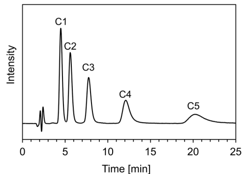
Fig. 3 Chromatogram of alkyl benzenes (C1: toluene; C2: ethylbenzene; C3: propylbenzene; C4: butylbenzene; C5: pentylbenzene) obtained with an ACSuc column. Analytical conditions: mobile phase: 100 mM citric acid buffer (pH 7)/methanol (90/10, v/v); column temperature: 40^\circ\text{C} ; flow rate: 0.2 \text{ mL min}^{-1} ; analyte concentration: 0.5 \text{ mg mL}^{-1} ; injection volume: 5 \mu\text{L} .
