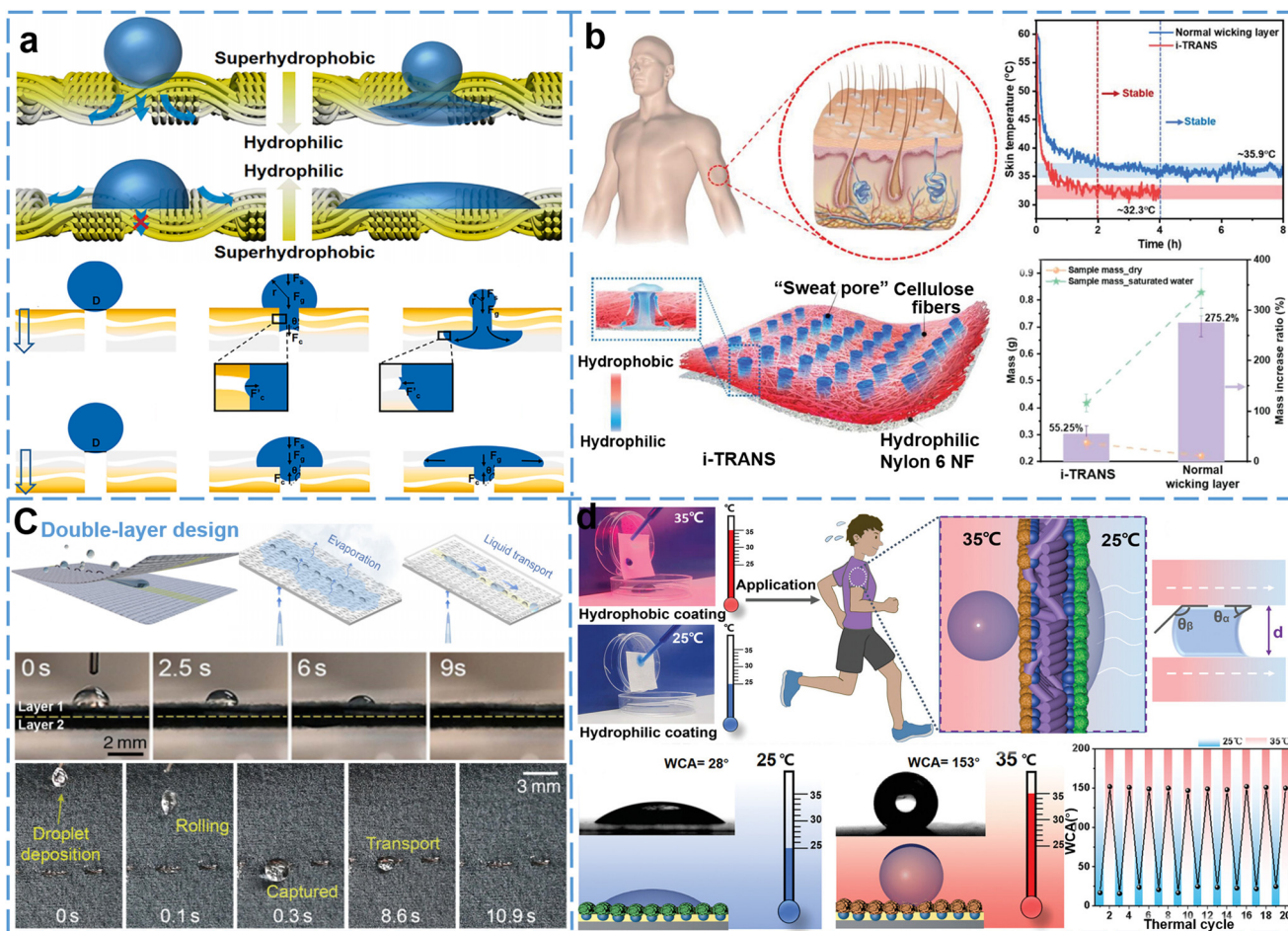
Fig. 9 (a) Janus fabric one-way water transport mechanism, 127 Copyright 2021 Elsevier; (b) concept illustration of integrated 3D hydrophilicity/hydrophobicity design for artificial sweating skin (i-TRANS), 169 Copyright 2022 Wiley-VCH; (c) schematic of the fabrication of the double-layer fabric assembly, 170 Copyright 2023 The Royal Society of Chemistry; (d) temperature triggered directional water transport fabric, 171 Copyright 2023 Wiley-VCH.
