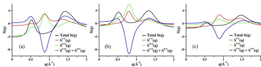
Fig. 2 Cation–cation, anion–anion, cation–anion, and total simulated S(q) for (a) N_{5,5,5,5}^+/PF_6^- , (b) N_{5,5,5,5}^+/PF_6^- , and (c) N_{5,5,5,5}^+/N(CN)_2^- in the liquid state. Reprinted 15 (adapted) with permission from J. Phys. Chem. Lett. , 2013, 4(1), 105–110. Copyright 2013 American Chemical Society.
