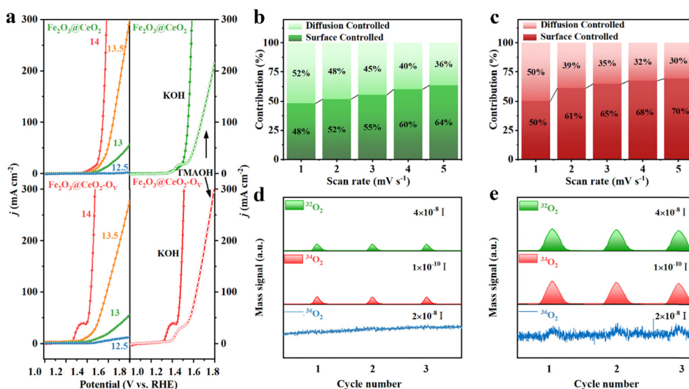
Fig. 5 OER performance of the prepared electrodes. (a) LSV curves of \text{Fe}_2\text{O}_3@/\text{CeO}_2-\text{O}_\text{V} and \text{Fe}_2\text{O}_3@/\text{CeO}_2 under different pH conditions (left) and in 1.0 M KOH or 1.0 M TMAOH, respectively (right). Contribution ratios of the capacitive and diffusion-controlled current densities vs. scan rates for (b) \text{Fe}_2\text{O}_3@/\text{CeO}_2 and (c) \text{Fe}_2\text{O}_3@/\text{CeO}_2-\text{O}_\text{V} . DEMS results by ^{18}\text{O} -isotopic labeling experiments for (d) \text{Fe}_2\text{O}_3@/\text{CeO}_2 and (e) \text{Fe}_2\text{O}_3@/\text{CeO}_2-\text{O}_\text{V} .
