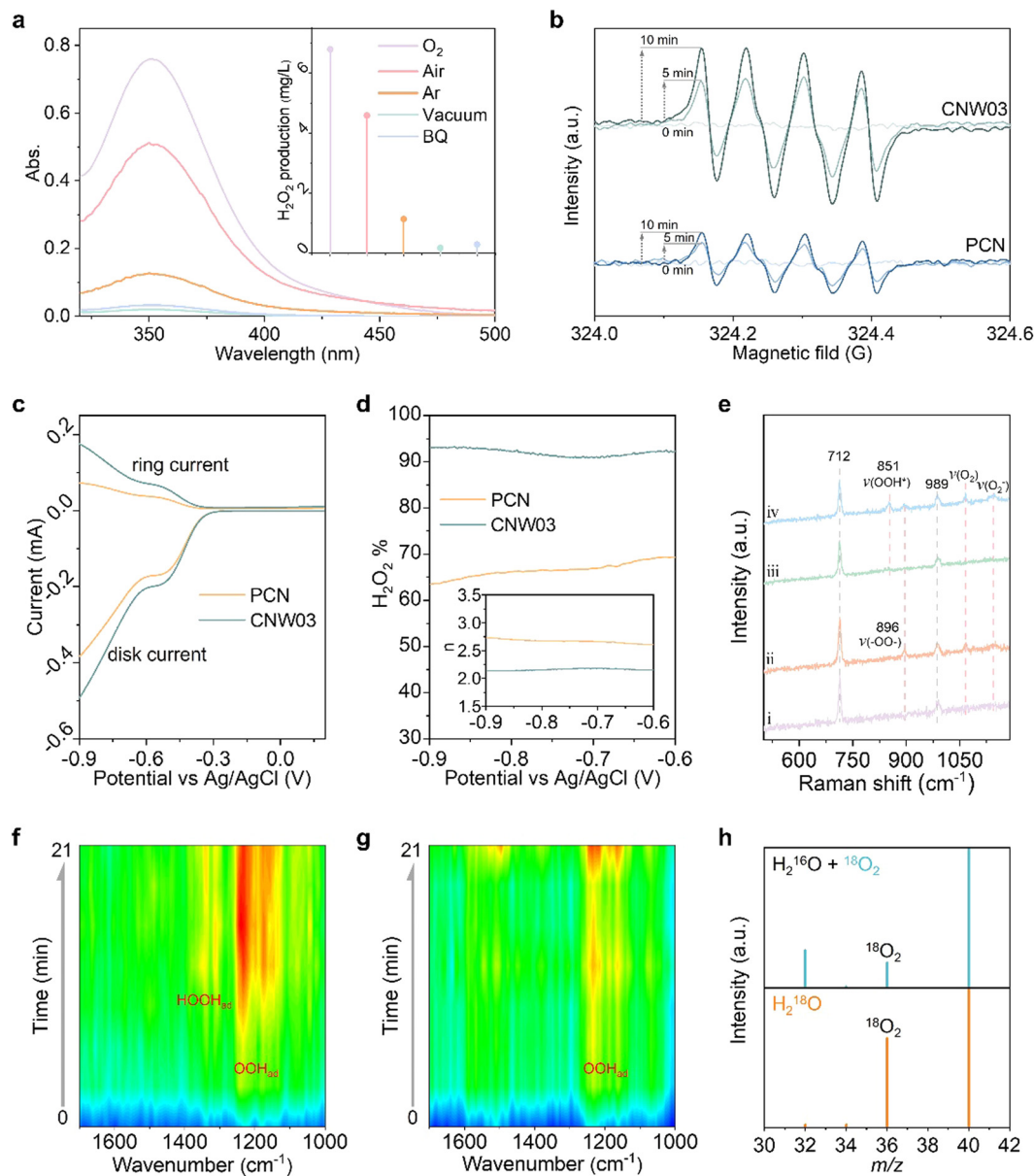
Fig. 5 (a) Photocatalytic \text{H}_2\text{O}_2 production over CNW03 with different reaction gases or sacrificial agents. (b) In situ EPR signals of DMPO- ^*\text{OOH} over PCN and CNW03 under visible light irradiation ( \lambda > 420\text{nm} , irradiation time: 0 min, 5 min and 10 min). (c) RRDE voltammograms of PCN and CNW03 in \text{O}_2 -saturated solution. (d) Percentage of peroxide and the electron transfer numbers (inset) of PCN and CNW03 at various potentials. (e) Raman spectra for PCN and CNW03 recorded after 2 h of visible light irradiation in an \text{O}_2 -saturated propanol/water mixture. (i) PCN before irradiation, (ii) PCN after irradiation, (iii) CNW03 before irradiation, and (iv) CNW03 after irradiation. In situ DRIFT spectra of \text{O}_2 photocatalytic reduction over (f) CNW03 and (g) PCN. (h) GCMS spectra of \text{O}_2 transformed from \text{H}_2\text{O}_2 formed by \text{H}_2^{16}\text{O} + ^{18}\text{O}_2 (upper) or \text{H}_2^{18}\text{O} (lower).
