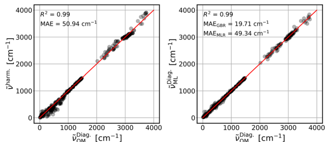
Fig. 3 Left panel: QM calculated diagonal frequencies ( \hat{\nu}_{\text{QM}}^{\text{Diag}} ) vs. harmonic frequencies ( \hat{\nu}^{\text{harm}} ); right panel: QM calculated diagonal frequencies ( \hat{\nu}_{\text{QM}}^{\text{Diag}} ) vs. ML predicted diagonal frequencies ( \hat{\nu}_{\text{ML}}^{\text{Diag}} ). \hat{\nu}_{\text{ML}}^{\text{Diag}} are LOOCV GBR predictions. Red lines are ideal diagonals.
