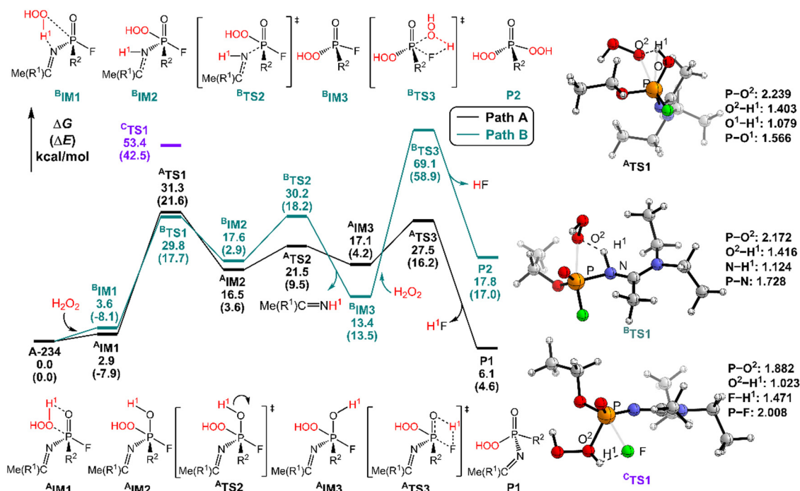
Fig. 2 Predicted relative free energy profiles ( \Delta G in kcal mol ^{-1} ) and electronic energies ( \Delta E in parentheses) of the species involved in the perhydrolysis of A-234 by H_2O_2 . The main transition state structures and the selected key bond lengths (in Å) are given.
