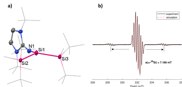
Fig. 2 (a) Molecular structure of silyl radical 2 (left) with thermal ellipsoids drawn at the 30% probability level. Hydrogen atoms are omitted for clarity, t\text{Bu} - and \text{Me} -groups are simplified as wireframes. Selected bond lengths [Å] and angles [°]: Si1–Si2 2.3843(7), Si1–Si3 2.3790(8), Si1–N1 1.676(2), N1–C1 1.280(3), Si2–Si1–Si3 132.98(3), Si3–Si1–N1 108.91(7), N1–Si1–Si2 111.62(7). (b) X-Band EPR spectrum (right) of 2 in n -hexane ( 2 \times 10^{-3}\text{ M} ) at 286 K; (black) experimental, (red) simulation.
