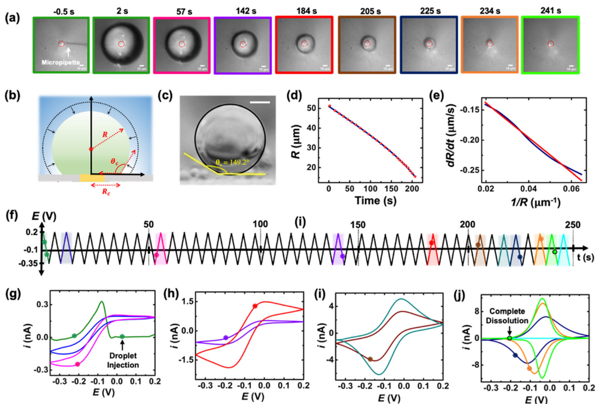
Fig. 3 (a) Optical micrographs recorded during the dissolution of a 51 μm radius droplet containing 155 μM of (Cp*) 2 Fe II in a 10 mM NaClO 4 aqueous bulk phase. The solid red line incrustated in the micrographs indicates the position of the gold-disk electrode. The scale bar is 10 μm. (b) Side-view schematic of the droplet sitting on the electrode. (c) Side-view optical micrograph of a DCE droplet on a glass surface and immersed in water. The scale bar represents 10 μm. (d) Apparent droplet's radius as a function of time measured from the optical micrographs in (a). The data points shown in red represent the apparent radius of the droplet measured using the acquired micrographs. The solid blue curve represents a polynomial fit used to obtain a smooth representation of the data points. (e) Normal velocity of the water|DCE as a function of the inverse of the droplet's radius. The solid navy curve is a linear fit on the data, slope = -2.4 \pm 0.003 \text{ cm}^2 \text{ s}^{-1} , R^2 = 0.992 . (f) Potential ramp applied during the dissolution of the droplet shown in (a). The colored segments in the potential ramp function correspond to the colored segments of the voltammogram in (g)–(j). Panels (g)–(j) show cyclic voltammograms recorded simultaneously with the optical micrographs during the dissolution of the DCE droplet at a scan rate of 0.2 \text{ V s}^{-1} . The color code used for the cyclic voltammograms matches the color code in (f). The points on the cyclic voltammogram indicate the exact time when the frames in (a) were taken. The voltammograms were smoothed using adjacent weighted averaging with 19 points per window and a Savitzky–Golay algorithm with 32 points per window, and a periodic boundary condition. See Fig. S4† for an overlay of experimentally obtained CV and noise filtered CV of the purple curve in (h).
