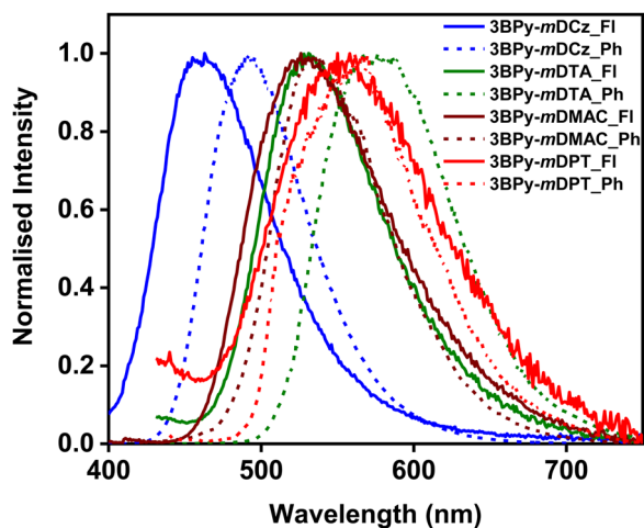
Fig. 3 Fluorescence (FI) and phosphorescence (Ph) spectra of 7 wt% 3BPY-mDCz :DPEPO, 3BPY-mDTA :mCBP, 3BPY-mDMAC :mCBP and 3BPY-mDPT :mCBP doped film.
