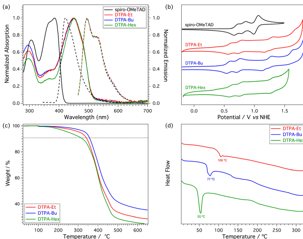
Fig. 4 (a) UV-Vis absorption spectra (solid line) and fluorescence emission spectra (dashed line) of DTP-based HTMs in \text{CH}_2\text{Cl}_2 . (b) Cyclic voltammety of DTP-based HTMs recorded in \text{CH}_2\text{Cl}_2 containing 0.1 M tetrabutylammonium hexafluorophosphate (TBAPF 6 ) at a scan rate of 100 \text{ mV s}^{-1} . (c) TGA curves recorded for DTP-based HTMs under nitrogen at a heating rate of 10 \text{ °C min}^{-1} . (d) DSC curves of DTP-based HTMs under nitrogen at a heating rate of 20 \text{ °C min}^{-1} (second cycle).
