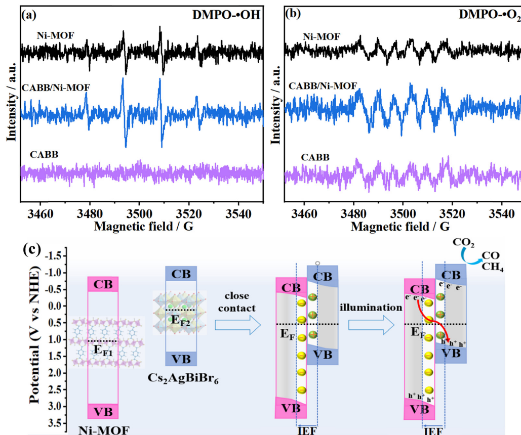
Fig. 7 ESR spectra of CABB NSs, Ni-MOF NSs, and the CABB/Ni-MOF hybrid for the detection of (a) DMPO- \cdot OH and (b) DMPO- \cdot O _2^- ; (c) schematic illustration of the formation process of the S-scheme heterojunction between CABB NSs and Ni-MOF NSs.
