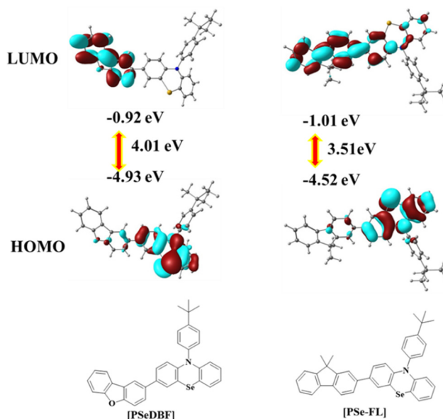
Fig. 1 Frontier orbitals distributions of PSeDBF and PSeFL.
