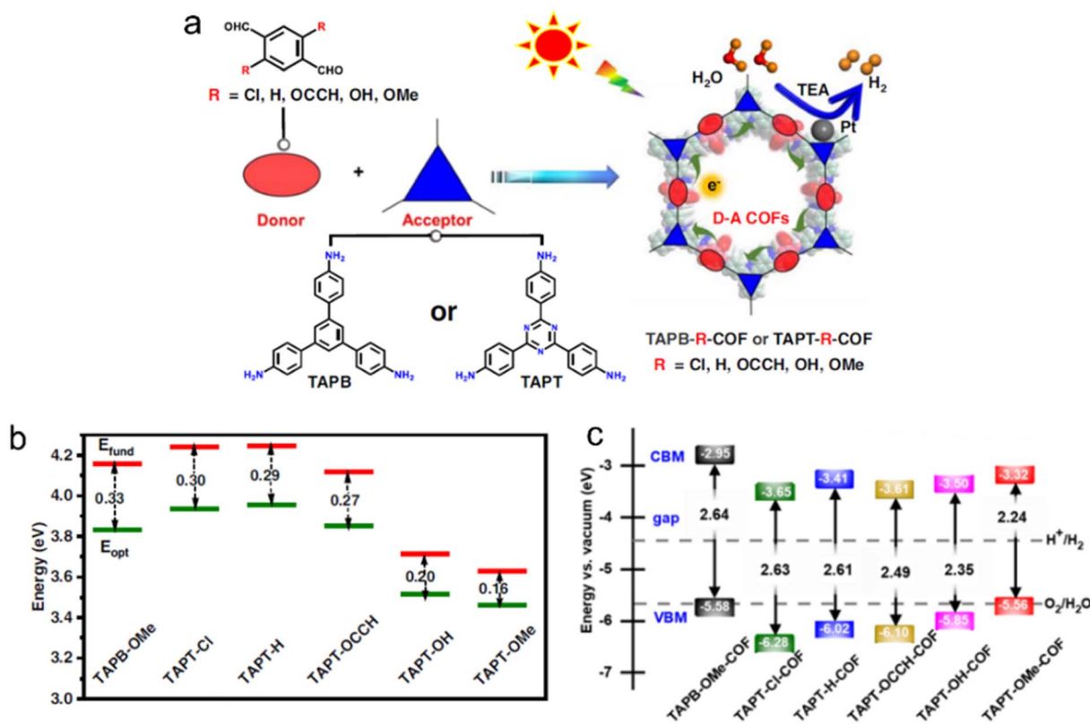
Fig. 10 (a) D-A COFs constructed from amine monomers and functionalized tereph-thaldehydes for photocatalytic H 2 evolution under a 300 W Xe lamp ( \lambda > 380 nm) by using triethylamine as a sacrificial agent. TAPB, TAPT and TEA indicate 1,3,5-tris(4-aminophenyl)benzene, 1,3,5-tris(4-aminophenyl)triazine and triethylamine, respectively. (b) Extrapolation results of fundamental gap ( E_{fund} , red line) and optical gap ( E_{opt} , green line) energies of D-A pairs. E_b (exciton binding energy) = E_{fund} - E_{opt} . (c) The calculated bandgap and band position of COFs relative to the vacuum level. The dashed lines are the redox potential of water at pH = 0. Reproduced with permission from ref. 100 . Copyright 2023, Springer Nature.
