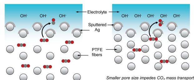
Scheme 1 CO 2 mass transport through the gas diffusion layer is slower with a smaller GDL pore size. This results in a higher local pH, which then induces a higher selectivity towards formate. Note: items in the schematic are not drawn to scale.
