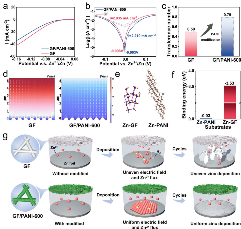
Fig. 4 (a) LSV curves at a scan rate of 5.0 mV s -1 and (b) Tafel plots of the Zn||Zn symmetric batteries with different separators. (c) The calculated transfer number of zinc ions ( t Zn 2+ ). (d) The electrical field distribution on the GF and GF/PANI-600 separators. (e) Optimized adsorption configurations and (f) the corresponding binding energy of GF and PANI-600 with Zn. (g) The schematic demonstration of the evolution of the plating process on Zn anodes with GF/PANI-600 and pristine GF separators.
