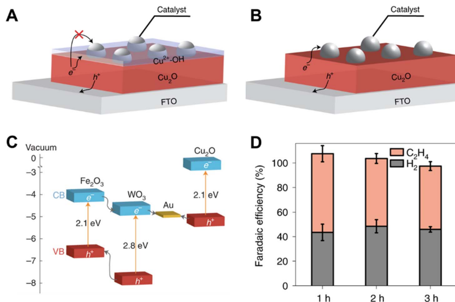
Fig. 4 (A) Schematic of the charge transfer between Cu 2 O and the catalysts, in the presence of Cu 2+ -OH (aq) species. (B) Schematic of the charge transfer between Cu 2 O and the catalysts, in the absence of Cu 2+ -OH (aq) species. (C) The band diagram of suitable candidates for constructing the Z-scheme system. (D) Faradaic efficiencies on the Ag/Cu 2 O/ZS/FTO photocathode for CO 2 R over time at -1.2 V versus Fc + /Fc under AM 1.5G simulated sunlight (100 mW cm -2 ) using 0.1 M Bu 4 NPF 6 as the electrolyte and 0.1 M TEOA as the proton donor in AcCN solution (CO 2 saturated). 40 Copyright 2021, Springer Nature.
