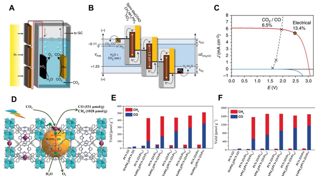
Fig. 7 (A) Schematic illustration of the device combining photovoltaics with an electrochemical cell. (B) Generalized energy diagram for converting CO 2 into CO with three perovskite solar cells connected in series, (C) J – V curves of three series-connected perovskite cells under simulated AM 1.5G 1 Sun solar irradiation and in the dark, overlaid with the matched J – V characteristic of the CO 2 -reduction and oxygen-evolution electrodes. The maximum power point of the photovoltaics is indicated by the circled red dot on the curve. 57 Copyright 2015, Springer Nature. (D) Schematic diagram of CO 2 photoreduction over the MAPbI 3 @PCN-221(FeO 2 ) photocatalyst, photocatalytic performance: yield of the CO 2 reduction to CH 4 and CO in the CO 2 -saturated ethyl acetate/water solution after (E) 25 h and (F) 80 h. 58 Copyright 2019, Wiley.
