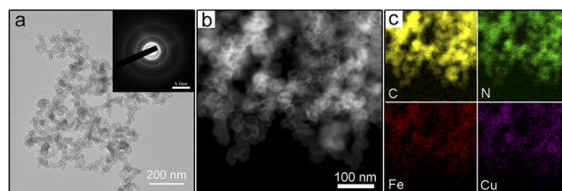
Fig. 1 (a) TEM and SAED (insert) images of FeCu-SAC. (b) HAADF-STEM image of FeCu-SAC. (c) EDX elemental maps of FeCu-SAC.
