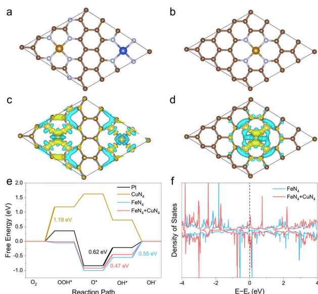
Fig. 4 (a) Optimized structure of FeCu-SAC. (b) Optimized structure of Fe-SAC. (c) Electron density difference analysis of FeCu-SAC. (d) Electron density difference analysis of Fe-SAC. (e) Calculated free-energy evolution diagram for ORR of Pt, Fe-SAC, Cu-SAC and FeCu-SAC at 1.23 V. (f) Density of states for FeN 4 + CuN 4 and FeN 4 .
