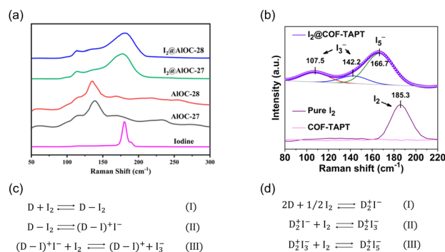
Fig. 4 (a) Raman spectra of AIOC-27, AIOC-28, I_2@AIOC\text{-}27\text{-NC} , I_2@AIOC\text{-}28\text{-NC} , and solid I_2 . In the spectra of I_2@AIOC\text{-}27\text{-NC} and I_2@AIOC\text{-}28\text{-NC} , the peak at 180 \text{ cm}^{-1} assigned to solid I_2 was red-shifted, indicating the formation of neutral charge transfer complex D \cdot I_2 . Reproduced with permission from ref. 73. Copyright 2021, American Chemical Society. (b) Raman spectra of pure I_2 , pristine COF-TAPT, and I_2 -saturated COF-TAPT. In the spectra of I_2@COF\text{-TAPT} , peaks attributed to I_3^- and I_5^- appeared, indicating the formation of charged polyiodides in COF-TAPT. Reproduced with permission from ref. 99. Copyright 2022, Springer Nature. (c and d) The interaction mechanisms between electron donors and I_2 proposed by different researchers. 58–62
