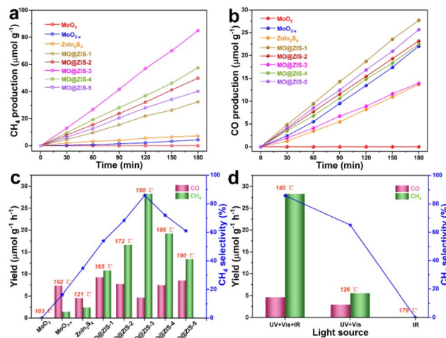
Fig. 6 (a) CH 4 production and (b) CO production as a function of irradiation time under full-spectrum illumination over the prepared samples. (c) Product yields, CH 4 selectivity and surface temperature of the as-prepared samples under full-spectrum illumination. (d) Product yields, CH 4 selectivity and surface temperature of the MO@ZIS-3 sample under different light irradiation.
