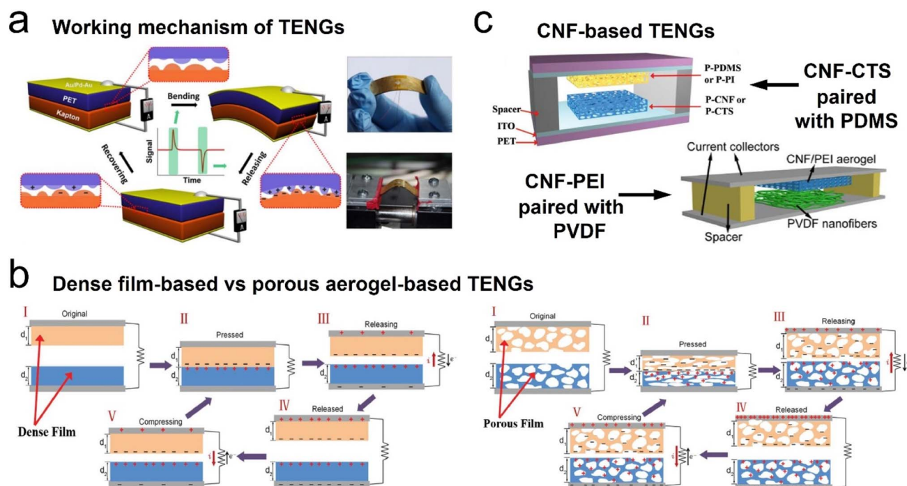
Fig. 16 Schematic illustration of the structure and working principle of the triboelectric generator. (a) Schematic illustration and working principle of TENGs. Reproduced with permission. 124 Copyright 2012, Elsevier. (b) Comparison of the surface charge density of dense film-based and porous aerogel-based TENGs. Reproduced with permission. 127 Copyright 2018, Wiley-VCH. (c) A schematic illustration of cellulose nanofibril-based TENGs: cellulose nanofibril–chitosan hybrid aerogels paired with PDMS or PI. Reproduced with permission. 127 Copyright 2018, Wiley-VCH. A schematic illustration of a cellulose nanofibril–polyethyleneimine (PEI) hybrid aerogel paired with PVDF. Reproduced with permission. 128 Copyright 2018, Elsevier.
