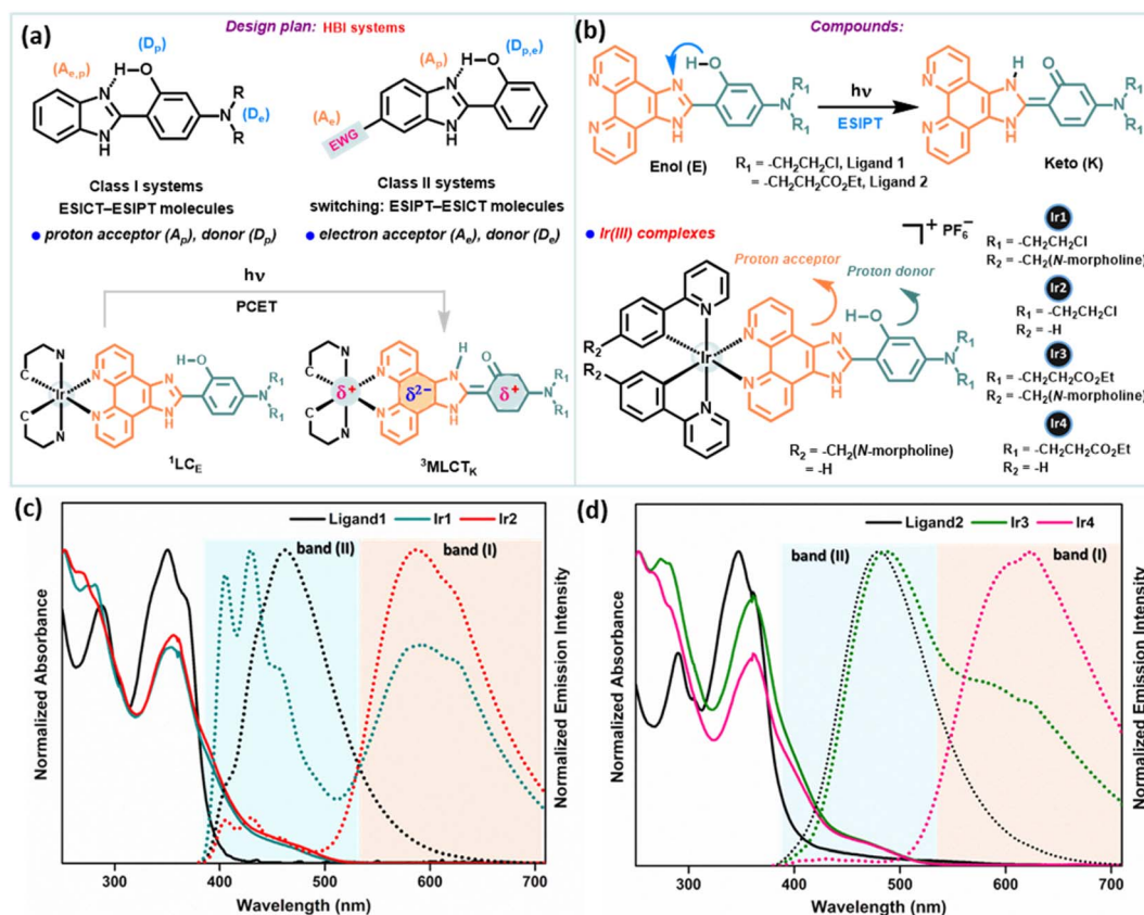
Fig. 2 (a) Design plan for synthesizing desired compounds. (b) Structures of phenanthroline-BIP based ancillary ligands attributing to the ESIPT phenomenon and the corresponding Ir(III)-complexes. The proton-accepting and donating parts are indicated in orange and cyan dark colors, respectively. (c) and (d) Normalized UV-vis absorption spectra (solid line) and the corresponding emission spectra (dotted line) of (c) ligand1, Ir1 and Ir2; (d) ligand2, Ir3 and Ir4; in DCM (10 \mu M), respectively under 365 nm excitation. Two emission bands are assigned as major band (I) and minor band (II), respectively.
