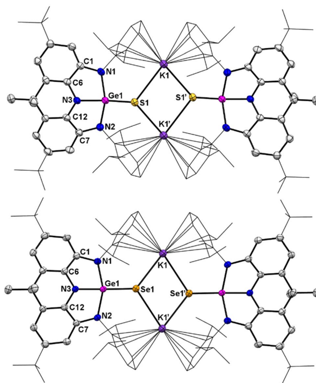
Fig. 6 Top: Solid-state structure of 6. Bottom: Solid-state structure of 7. The t Bu and Dipp groups are simplified as wireframes and hydrogen atoms are omitted for clarity. Thermal ellipsoids are set at the 30% probability level. Selected bond lengths (Å) and angles (°) for 6: Ge1–S1 2.1097(8), Ge1–N1 1.917(3), Ge1–N2 1.916(3), Ge1–N3 1.857(3), K1–S1 3.1094(11), K1–S1' 3.1491(10), C1–N1 1.394(4), C1–C6 1.394(4), C7–N2 1.396(4), C7–C12 1.395(4), C12–N3 1.403(4), N3–Ge1–S1 142.98(8), N1–Ge1–N2 139.16(11), N1–Ge1–N3 84.41(10), N2–Ge1–N3 84.41(10). Selected bond lengths (Å) and angles (°) for 7: Ge1–Se1 2.2595(12), Ge1–N1 1.928(3), Ge1–N2 1.934(3), Ge1–N3 1.872(3), K1–Se1 3.2541(17), K1–Se1' 3.2477(17), C1–N1 1.410(4), C1–C6 1.399(4), C7–N2 1.406(4), C6–N3 1.395(3), C12–N3 1.400(3), C7–C12 1.401(4), N3–Ge1–Se1 143.51(8), N1–Ge1–N2 140.30(11), N1–Ge1–N3 84.52(10), N2–Ge1–N3 83.59(10).
