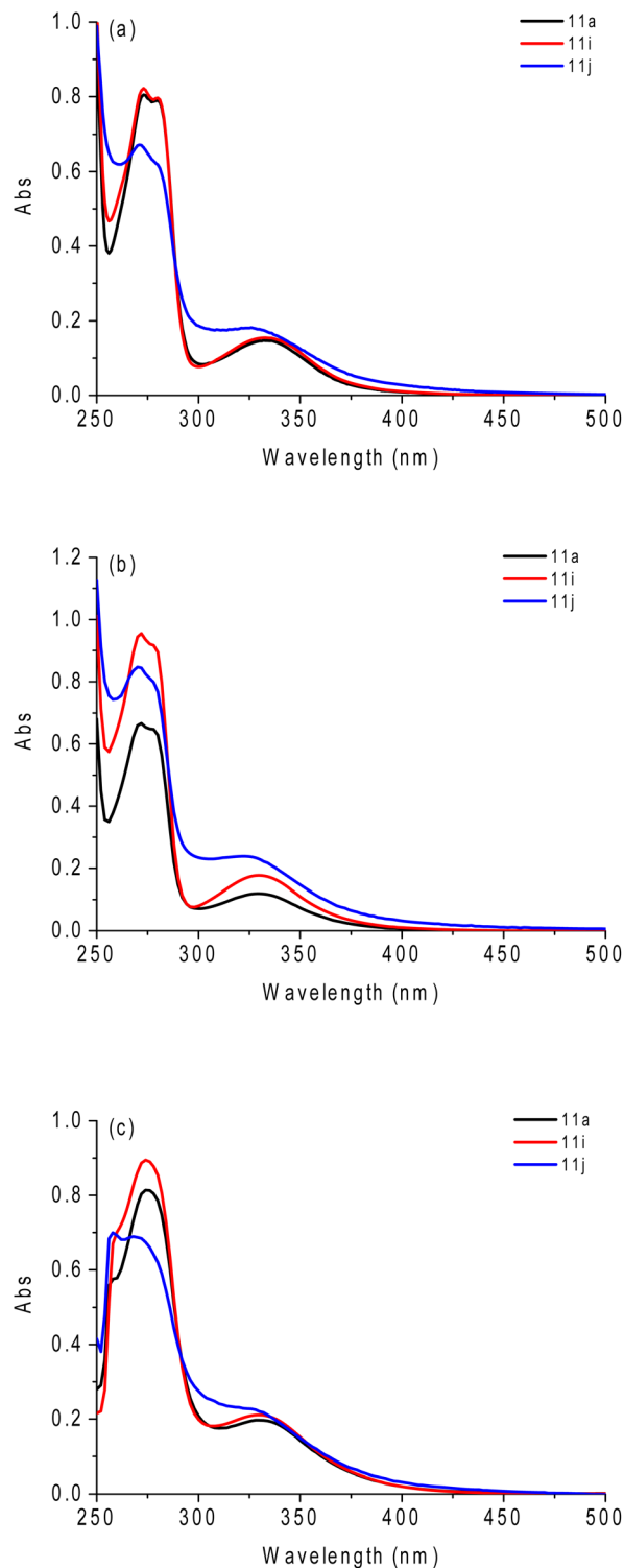
Fig. 3 Comparative absorption UV-vis spectra (concentration at 50 μM) of compounds 11a (Se atom), 11i (S atom) and 11j (Te atom) in (a) DCM, (b) ACN and (c) DMSO, respectively.
