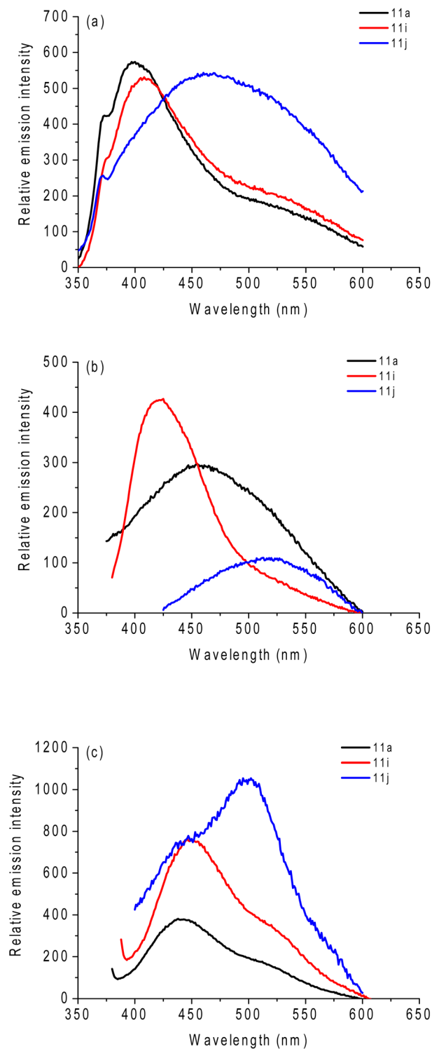
Fig. 4 Comparative steady-state fluorescence emission spectra (concentration at 5.0 μM) of compounds 11a (Se atom), 11i (S atom) and 11j (Te atom) in (a) DCM, (b) ACN and (c) DMSO, respectively. The compounds were excited in the higher energy transition band.
