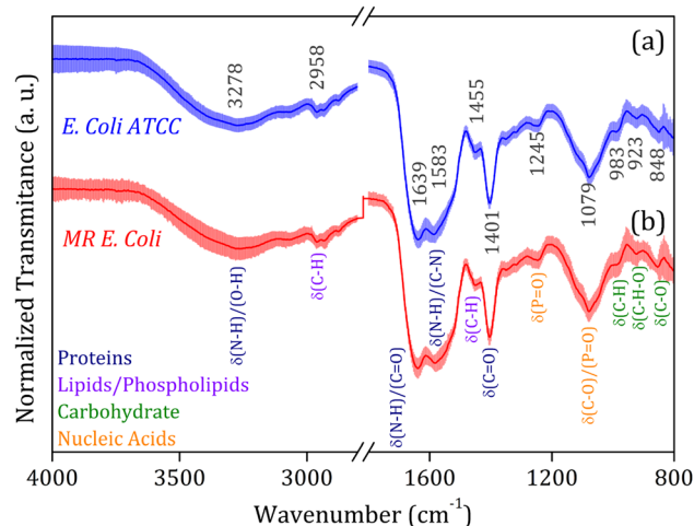
Fig. 2 Average FTIR-SNV spectra for (a) E. coli ATCC (blue line) and (b) multidrug-resistant (MR) E. coli isolates. The main vibrational assignments are indicated in detail, and their related molecular groups (proteins, lipids, carbohydrates, and fatty acids) are identified by colors. The symbol \delta indicates the deformation vibrations.
