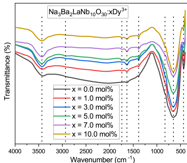
Fig. 8 Fourier transformed infrared (FT-IR) spectrum of \text{Na}_3\text{Ba}_2\text{LaNb}_{10}\text{O}_{30}:\text{x}\text{Dy}^{3+} ( x = 0, 1, 3, 5, 7 and 10 \text{ mol\%} ) phosphor at room temperature.
