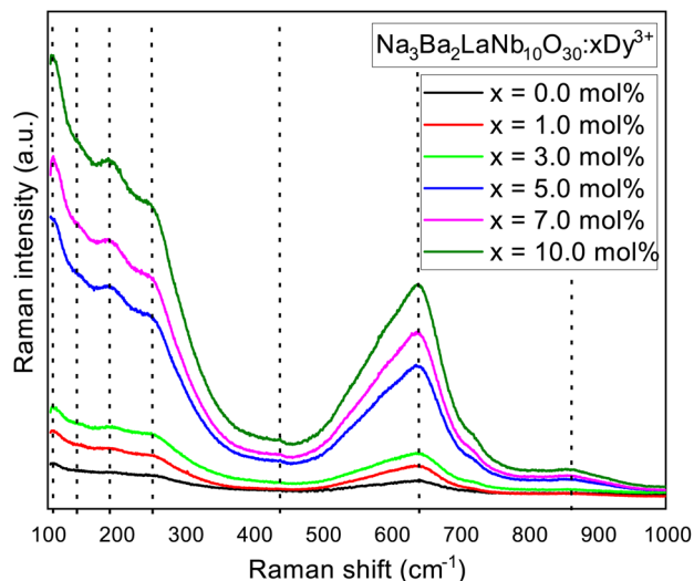
Fig. 7 Raman spectrum of \text{Na}_3\text{Ba}_2\text{LaNb}_{10}\text{O}_{30}:\text{x}\text{Dy}^{3+} ( x = 0, 1, 3, 5, 7 and 10 \text{ mol\%} ) phosphor at room temperature.
