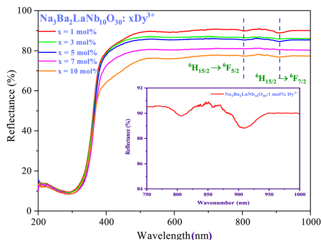
Fig. 9 Diffuse reflectance spectra of \text{Na}_3\text{Ba}_2\text{LaNb}_{10}\text{O}_{30}:\text{x}\text{Dy}^{3+} ( x = 1, 3, 5, 7 and 10 \text{ mol\%} ) phosphor.
