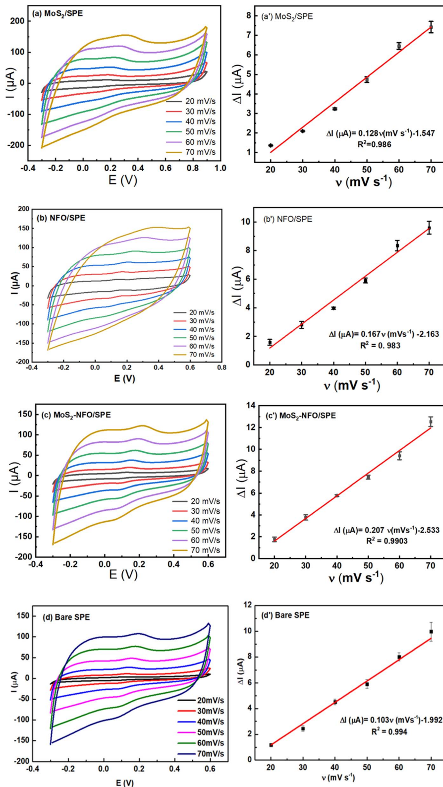
Fig. 5 CVs responses of 50 \mu\text{M} CLB at bare SPE (d), and the modified electrodes with \text{MoS}_2 (a), NFO (b), and \text{MoS}_2\text{-NFO} (2 : 1) (c) in 0.1 M PBS buffer at different scan rates; corresponding to the plot of peak current ( I ) versus scan rate ( \nu ) (a'–d').
