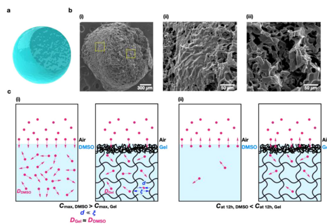
Fig. 3 (a) Schematic of a spherical ionic gel particle with the upper right portion removed for SEM measurements. (b) SEM images of the (i) entire structure of the ionic gel with a concentration of 5 wt%, (ii) reduced pore size at the interface, and (iii) increased internal pore size. The yellow dotted box indicates the magnified portion. (c) Schematic of the differences in the gas absorptions and retention mechanisms of DMSO and the gel (i) during the initial absorption and (ii) after 12 h. ( d : diameter of molecules, \xi : correlation length, D : diffusion coefficient).
