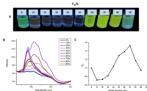
Fig. 7 (A) AIEE M2 samples under 366 nm to different THF/water ratios. (B) AIEE test emission spectrum. (C) plot of water fraction vs. I/I_0 .
