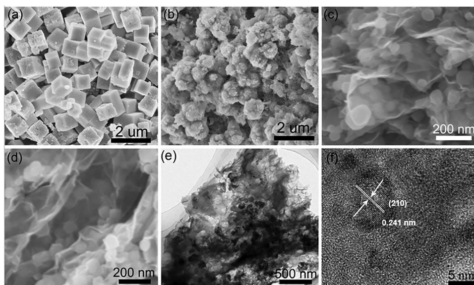
Fig. 11 SEM morphology of (a) PB, (b) \text{FeS}_2\text{-C} , (c) \text{PB/r-GO} , (d) \text{FeS}_2\text{-C/RG} , (e and f) TEM and HRTEM images of optimal \text{FeS}_2\text{-C/RG} . Reprinted with permission, 73 Copyright (2020) from Elsevier.
