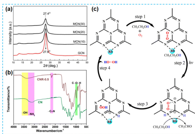
Fig. 4 (a) XRD patterns of K + –Na + codoped CN. 35 (b) FT-IR of CN and Rb doped CN (CNR-0.5). (c) Proposed mechanism of the two-step single-electron O 2 reduction reaction pathways on CNR-0.5. 36
