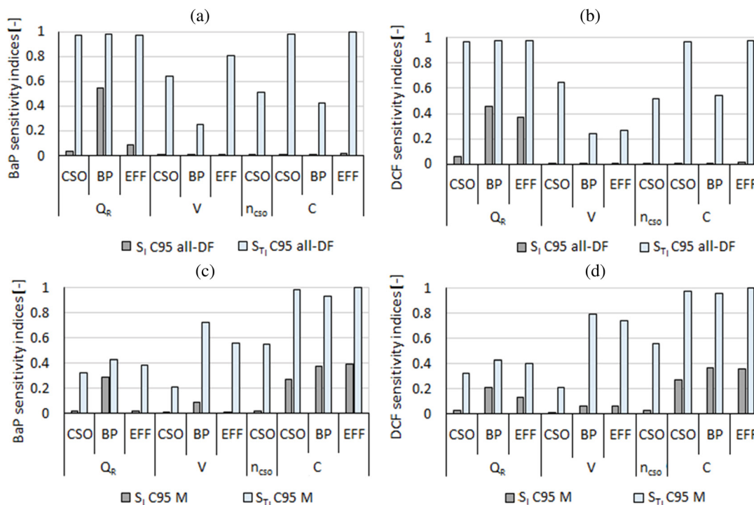
Fig. 7 S_1 (in grey) and S_{71} (in light blue) values for (a) BaP and (b) DCF in the all-DF scenario; in the medium scenario for (c) BaP and (d) DCF. Results refer to the scenario using the C95 distribution.
