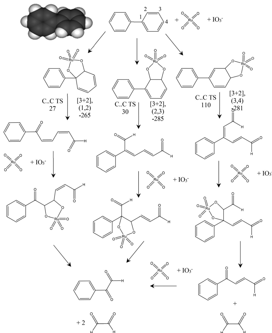
Fig. 5 Proposed mechanism for the oxidation of biphenyl using ruthenium tetroxide. [3 + 2] formation energies are quoted for the \text{Ru}^{\text{IV}} complex prior to oxidation with \text{IO}_3^- to the \text{Ru}^{\text{IV}} oxidation state form of the complex shown. Energies for C–C bond cleavage transition states (TS) are quoted for the forming \text{Ru}^{\text{IV}} state. Graphical inset shows the optimised geometry of biphenyl. Atom colours C: grey, H: white. All energies quoted in \text{kJ mol}^{-1} .
