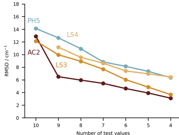
Fig. 10 RMSD values (in \text{cm}^{-1} ) for the four submissions with the lowest RMSD overall (PH5, AC2, LS3 and LS4). Note that the ordinate axis has a much smaller range than in the previous plots, with all four sets of values remaining below an RMSD of 15 \text{cm}^{-1} .
