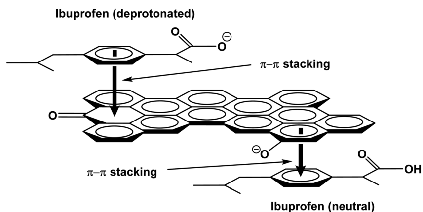
Scheme 6 \pi\text{-}\pi electron donor–acceptor attractions between neutral and deprotonated ibuprofen with aromatic rings on the WSAB surface.
