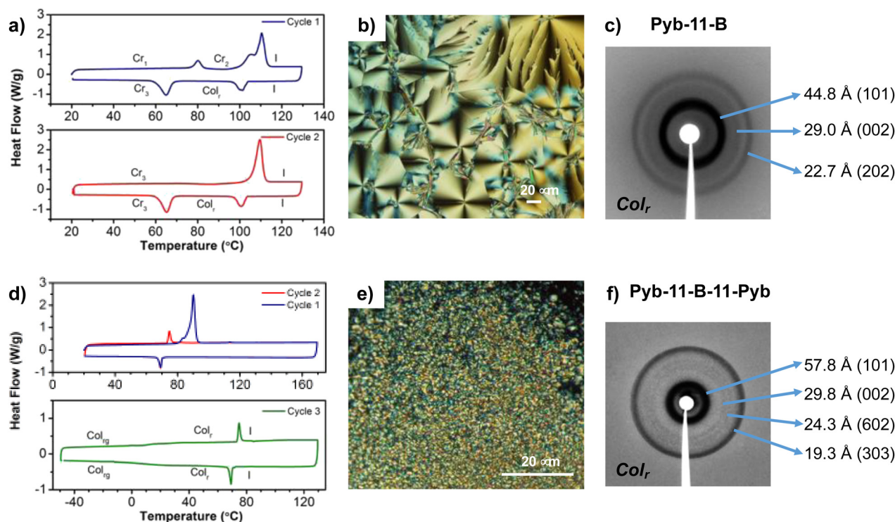
Fig. 2 DSC thermograms and first and second heating/cooling cycles of Pyb-11-B (a) and Pyb-11-B-11-Pyb (d); POM textures of Pyb-11-B at 104 ^{\circ}C (Col r phase) (b) and Pyb-11-B-11-Pyb at 74 ^{\circ}C (Col r phase) (e); and XRD patterns of the mesophases of Pyb-11-B, Col r phase at 102 ^{\circ}C , (c) and Pyb-11-B-11-Pyb, Col r phase at room temperature (f).
