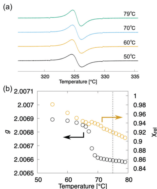
Fig. 6 EPR spectroscopy of (±)- 3 upon the cooling run. Black and orange circles denote the g -value and \chi_{\text{rel}} , respectively. Vertical dotted line denotes the N-to-N cyb phase transition point.
