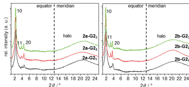
Fig. 5 2 \theta -scans along the equator and meridian of WAXS patterns of aligned fibres taken in the hexagonal phase at 150 °C of the 1:1, 1:2, and 1:3 mixtures of 2a and 2b with G2 .
