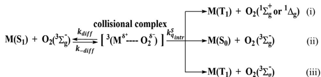
Scheme 3 The O 2 quenching S 1 state molecule M based on the spin conservation for the formation of the collisional complex.
