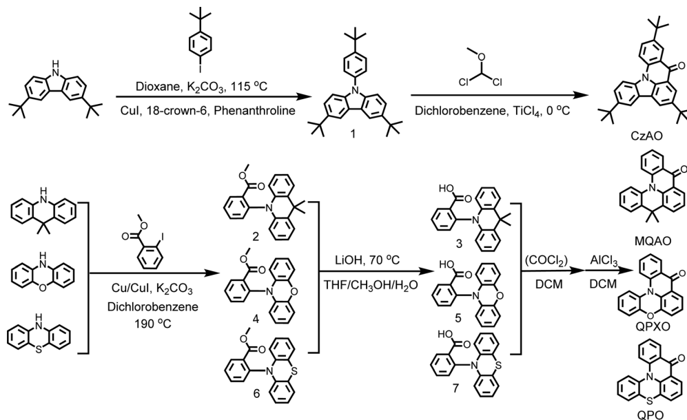
Scheme 2 Synthetic routes to CzaAO, MQAO, QPXO and QPO.
