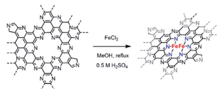
Scheme 2 Schematic representation of the proposed metalation reaction in C 2 N-like materials.
