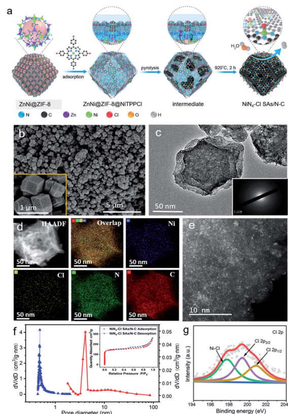
Fig. 1 (a) Synthetic scheme for \text{NiN}_4\text{-Cl SAs/NC} (b) SEM, (c) TEM, (d) EDS mapping, (e) AC-HAADF-STEM, (f) BET analysis and (g) Cl 2p XPS spectra of \text{NiN}_4\text{-Cl SAs/NC} .
