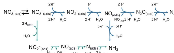
Fig. 9 The electron and absorbed hydrogen mediated direct electrocatalytic routes for the \text{NO}_3\text{RR} . Reproduced with permission from ref. 125. Copyright 2021 Elsevier.
