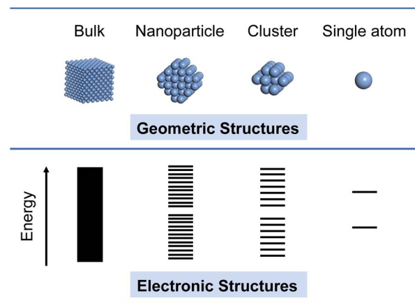
Fig. 1 Geometric and electronic structures of bulk, nanoparticles, clusters, and single atoms.
