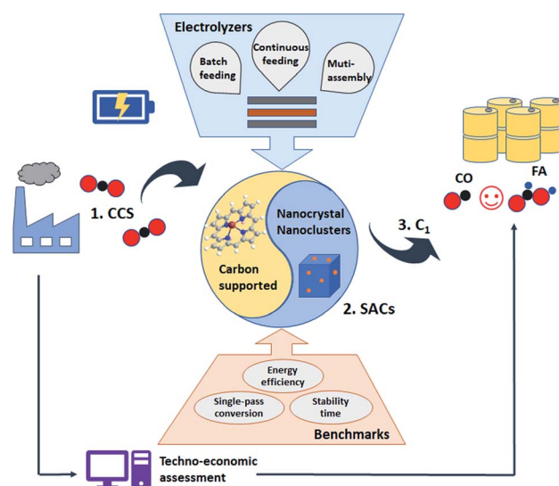
Fig. 1 Schematic of the whole industrial ECR process: the regulation of SACs is the crucial link for transferring \text{CO}_2 from carbon capture and storage (CCS) to \text{C}_1 products. Multi-assembly electrolyzer scales up the yield of \text{C}_1 . Through techno-economic assessment of the full lifecycle, the ECR performance satisfies the benchmarks, indicating that SACs are suitable for scaled-up use in industry.
