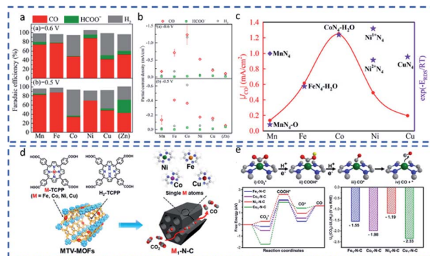
Fig. 3 (a) FE of the MNC catalysts ( \text{M} = \text{Mn}, \text{Fe}, \text{Co}, \text{Ni}, \text{and Cu} ) at -0.5\text{ V} and -0.6\text{ V} vs. RHE. (b) Volcano trend in partial current densities of MNC catalysts at -0.5\text{ V} and -0.6\text{ V} vs. RHE with the ECR in an H-cell. (c) Experimental CO partial current density and free reaction energy at RDS for MNC catalysts. Reprinted with permission from ref. 45 Copyright 2019, the American Chemical Society. (d) Schematic of the synthesis process of \text{M}_1-\text{N}-\text{C} catalysts ( \text{M} = \text{Fe}, \text{Co}, \text{Ni}, \text{and Cu} ) based on MOFs. (e) Free energy diagrams for \text{M}_1-\text{N}-\text{C} catalysts of \text{CO}_2 to CO with DFT calculation. Reprinted with permission from ref. 46 Copyright 2020, Wiley-VCH.
